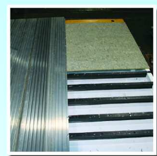
Composite Stringers, Composite Load plate, Steel Approach Plate
