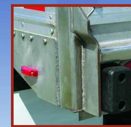
Impact Gusset and Bumper Blocks
